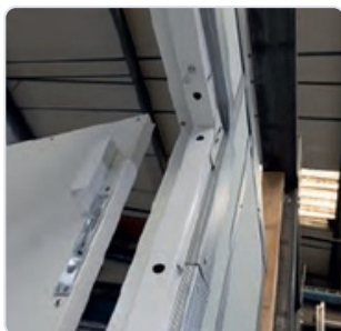
Quick release door mechanism operated by pull lever
